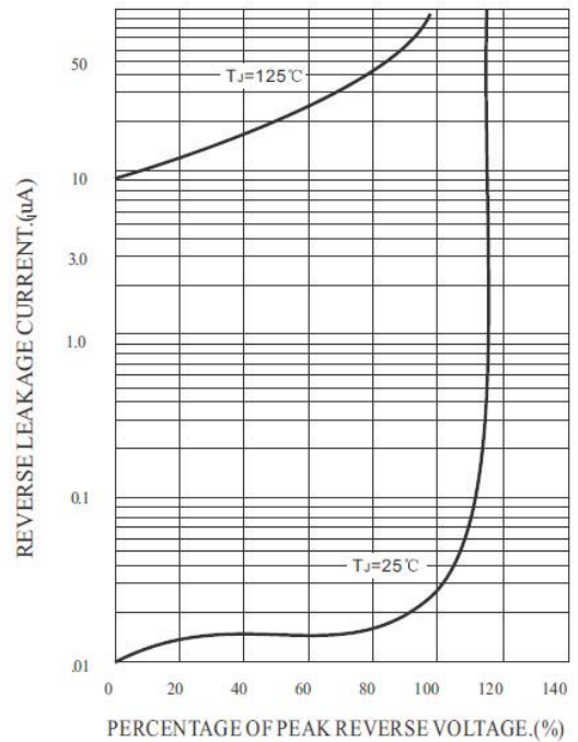
FIG.4-TYPICAL REVERSE CHARACTERISTICS
